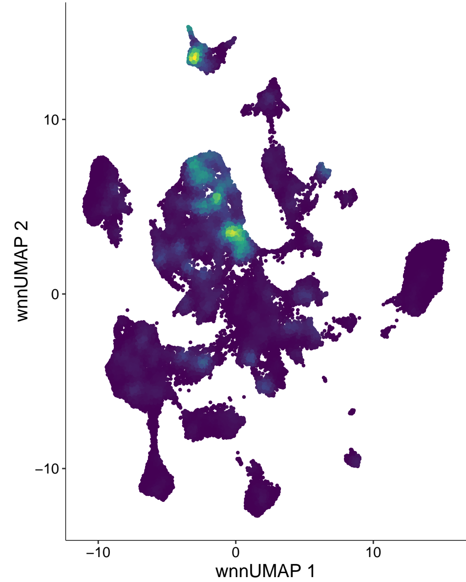
chr11-57419302-57419801
