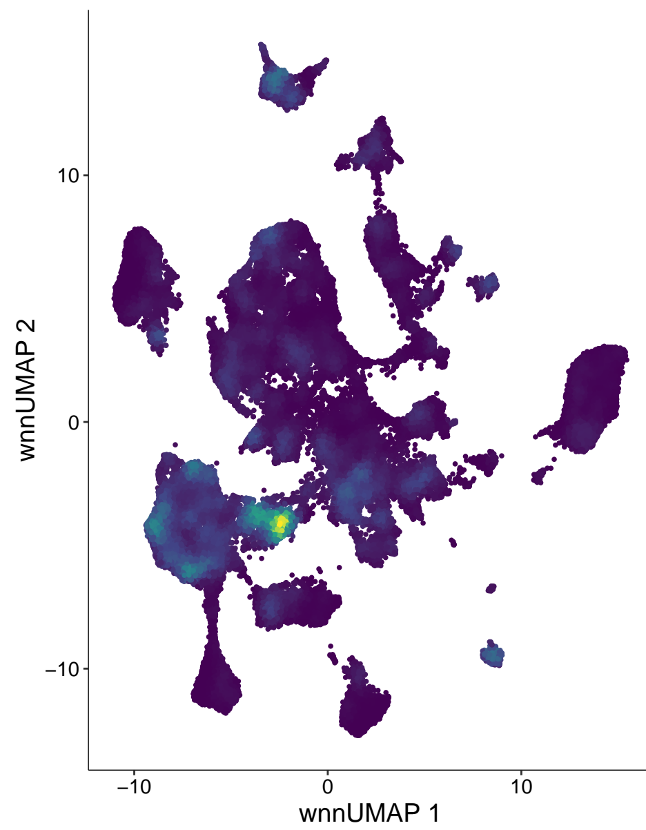
chr10-30733425-30733924
