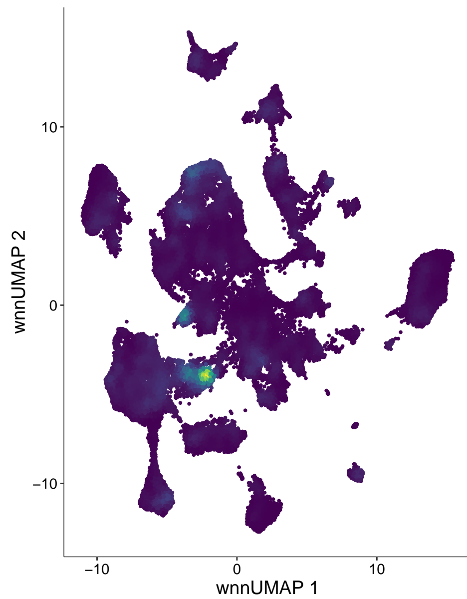
chr3-61842366-61842865
