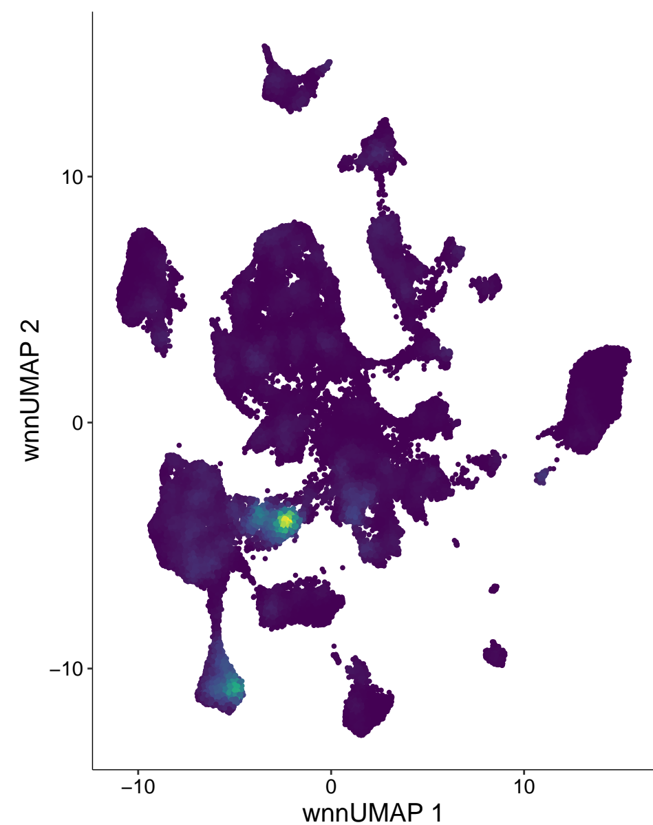
chr3-52822717-52823216
