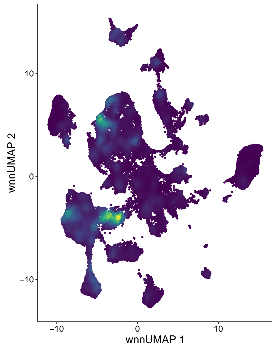
chr5-75963419-75963918
