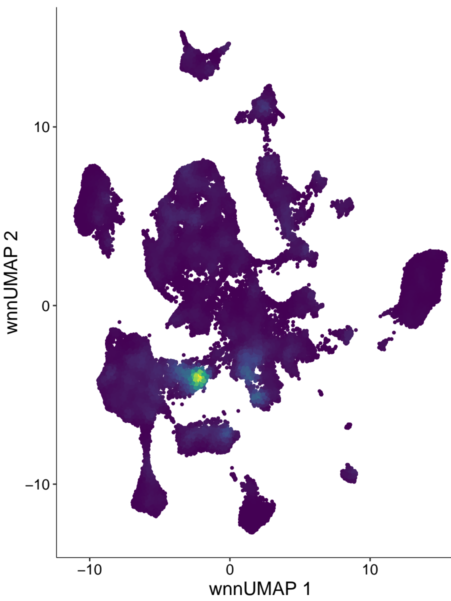
chr9-9007491-9007990
