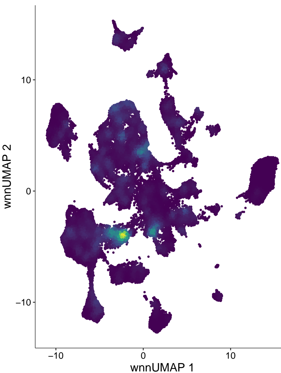
chr7-112970434-112970933
