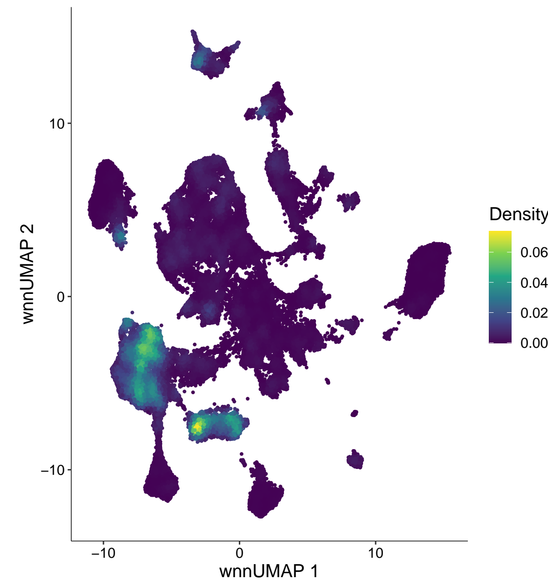
chr19-27385202-27385701
