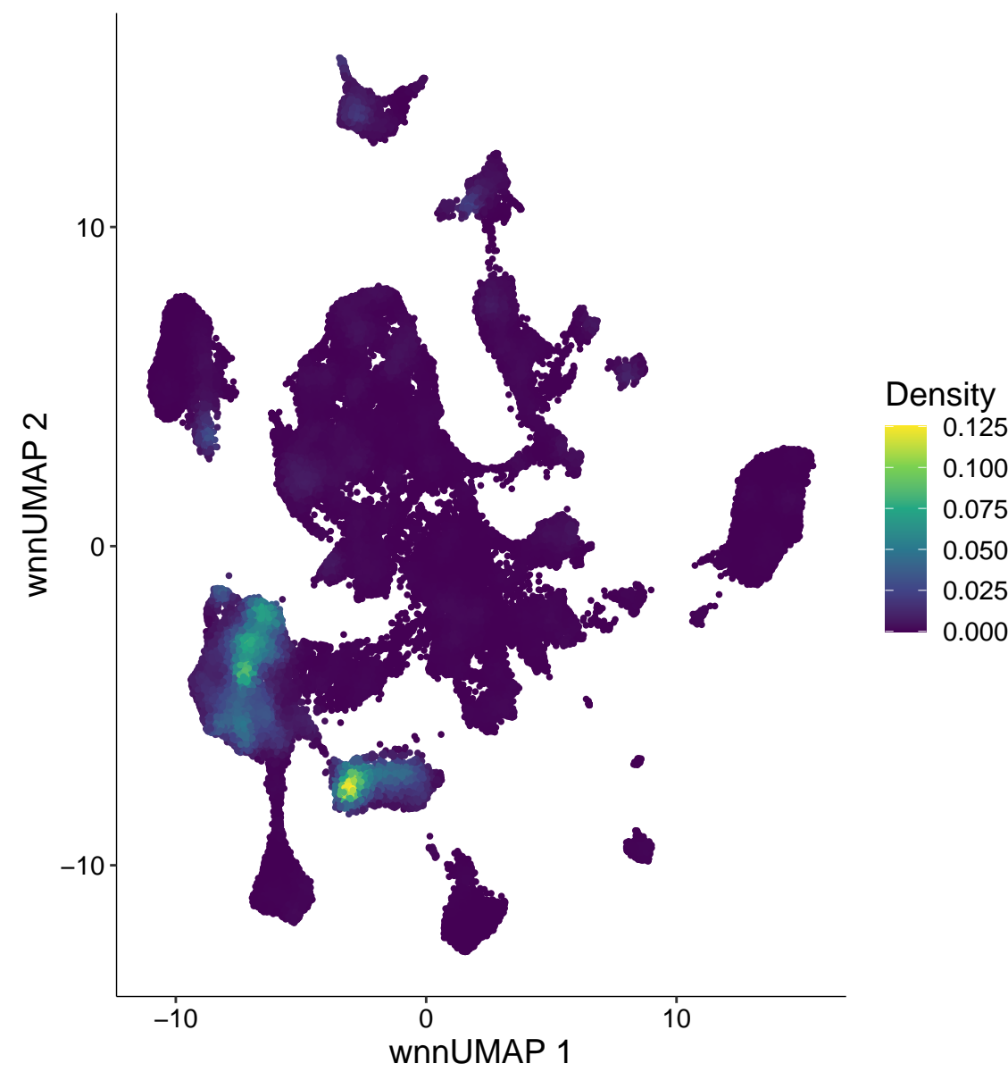
chr15-31753608-31754107
