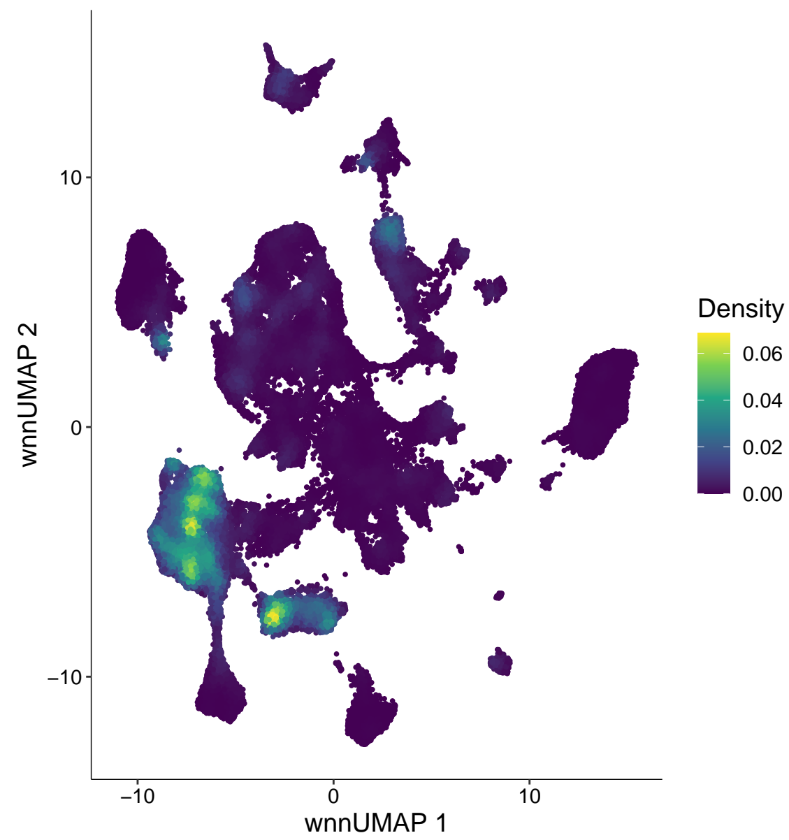
chr12-106734885-106735384
