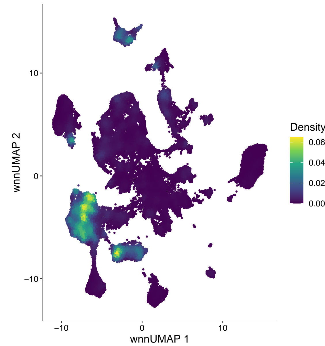
chr18-61835935-61836434
