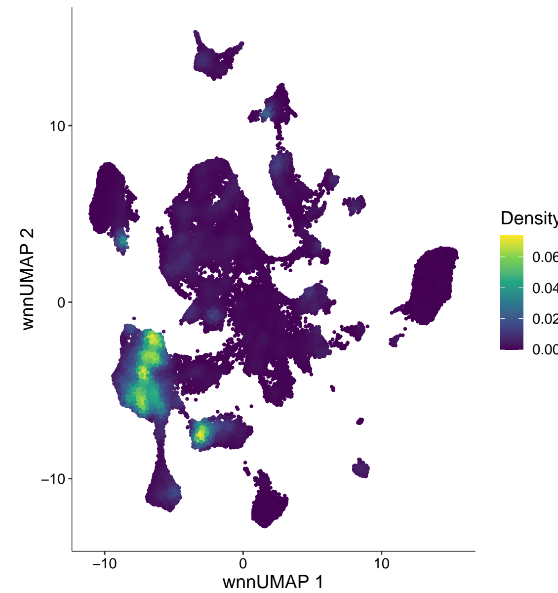
chr11-57573583-57574082
