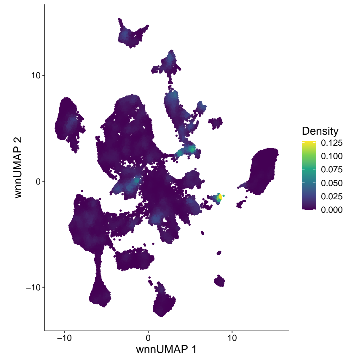
chr2-115249933-115250432
