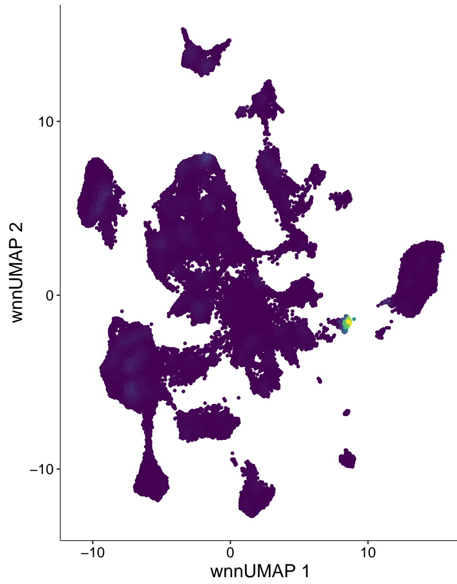
chr16-73244988-73245487
