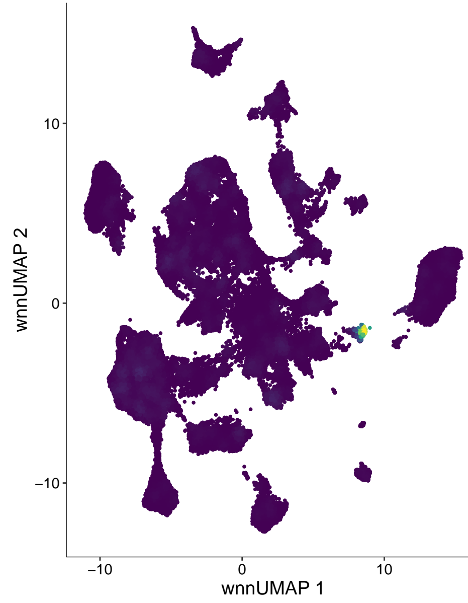
chr1-137838175-137838674
