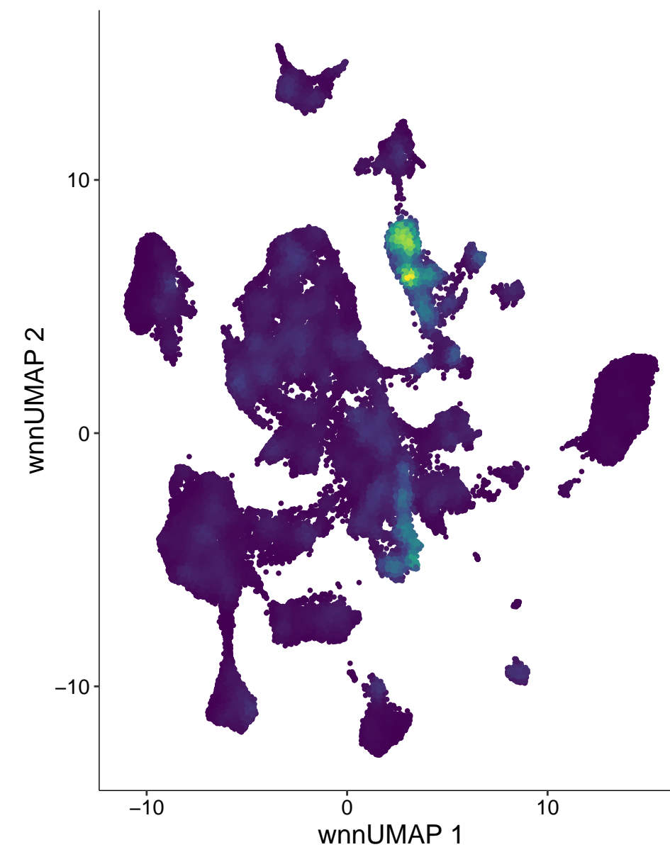
chr2-36202993-36203492
