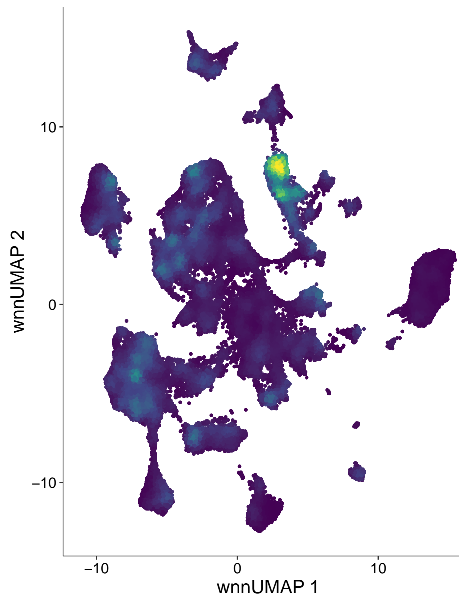
chr3-32924053-32924552
