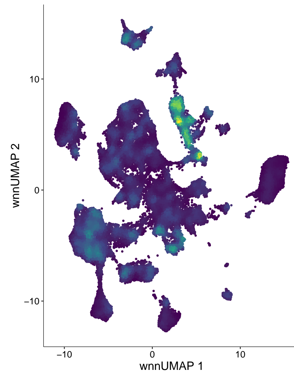
chr2-130351843-130352342
