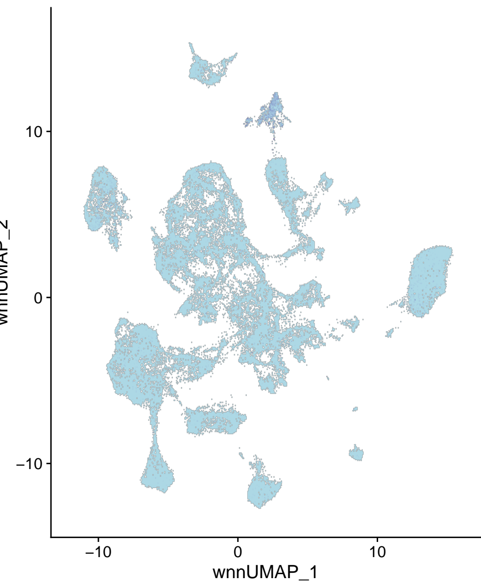
chr16-38673419-38673918
