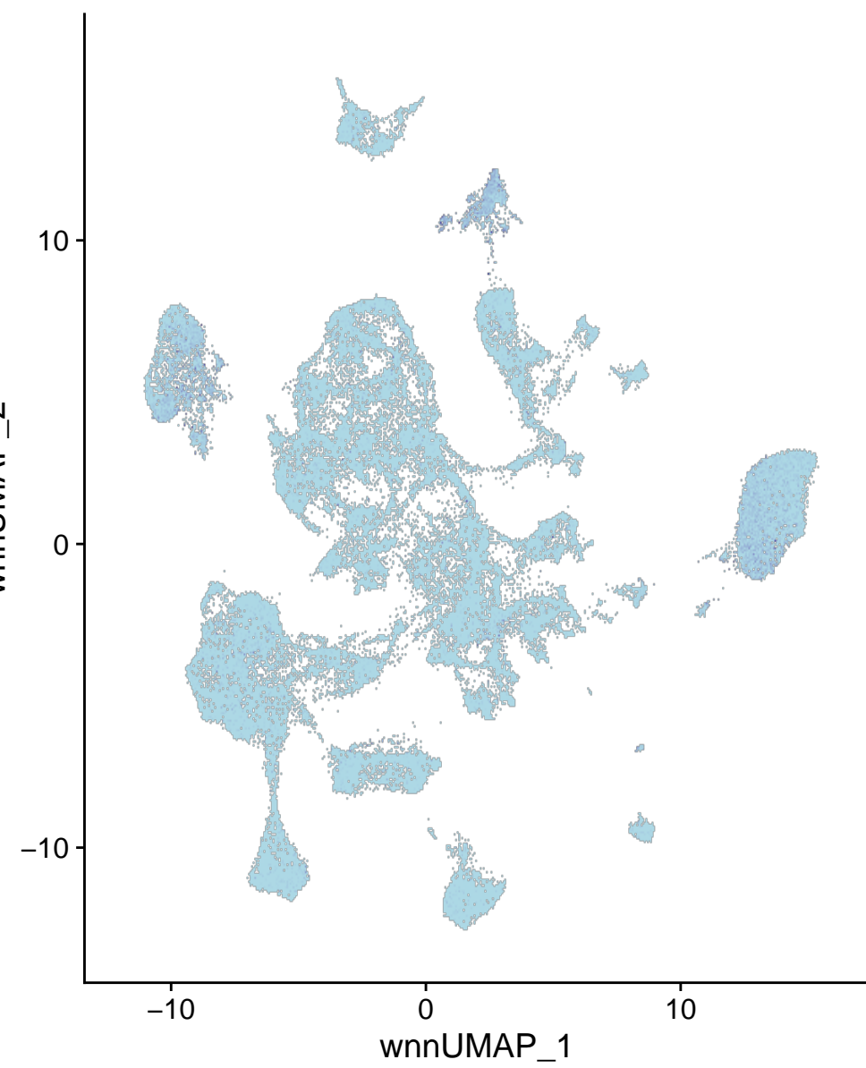
chr17-45733616-45734115
