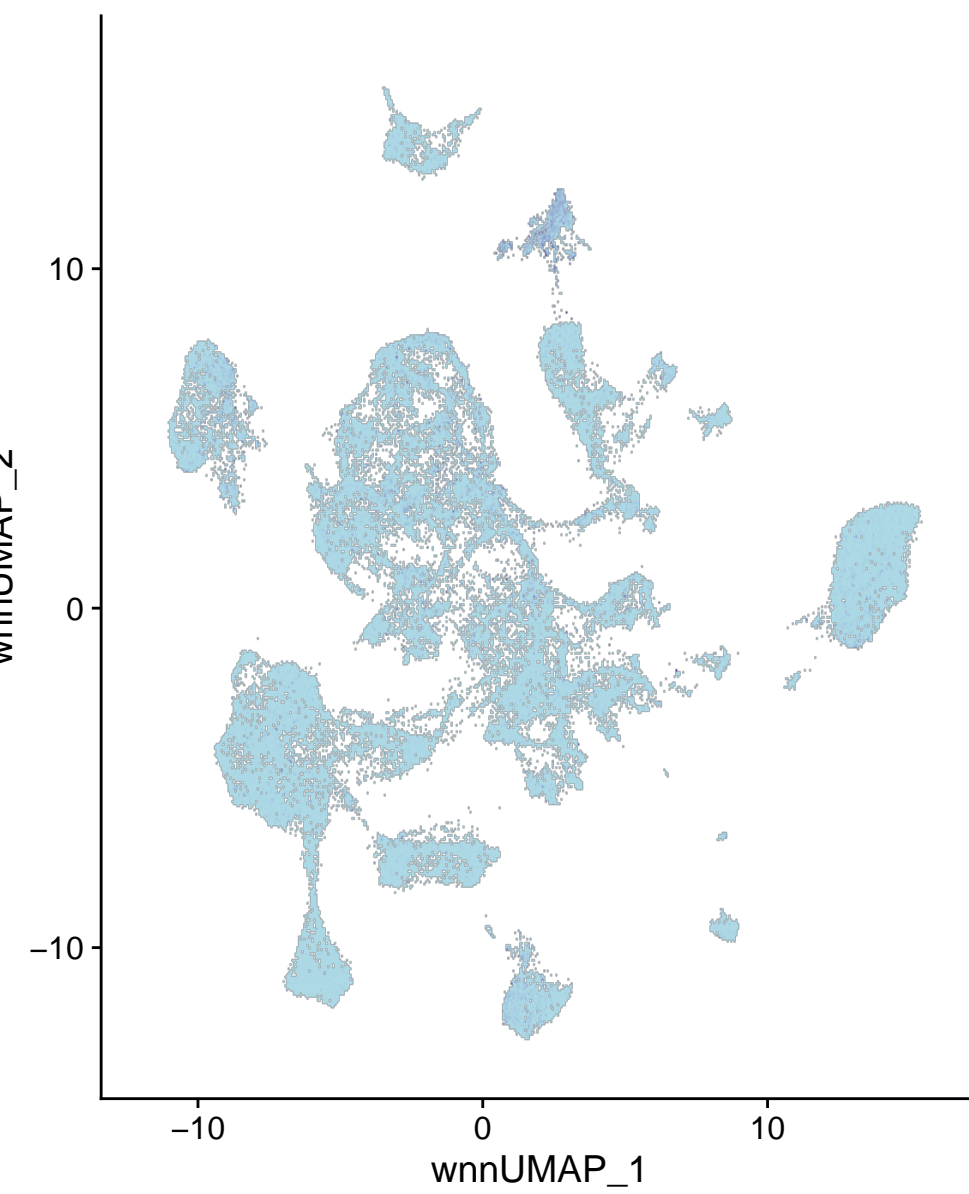
chr12-111693738-111694237
