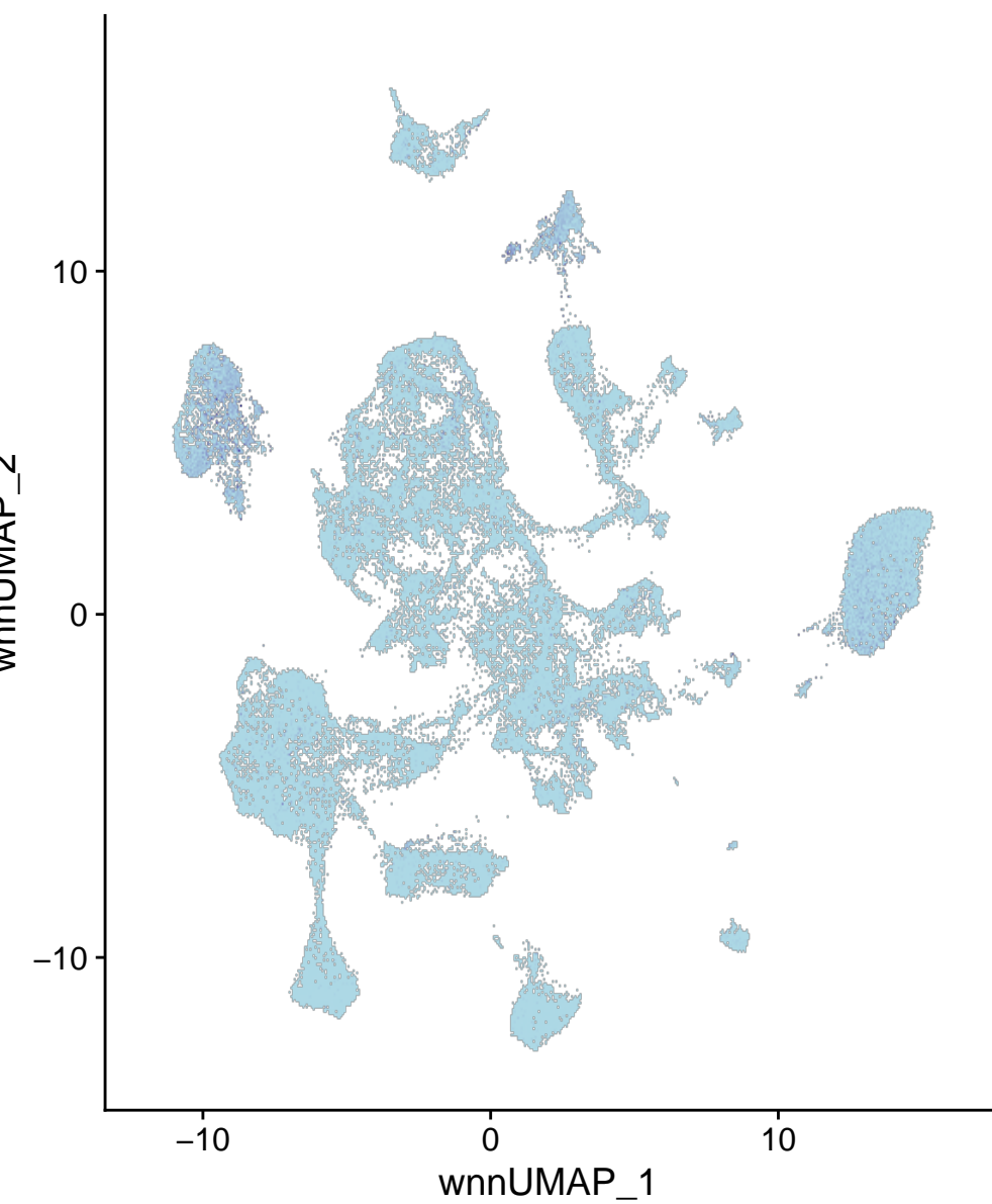
chr4-140657911-140658410
