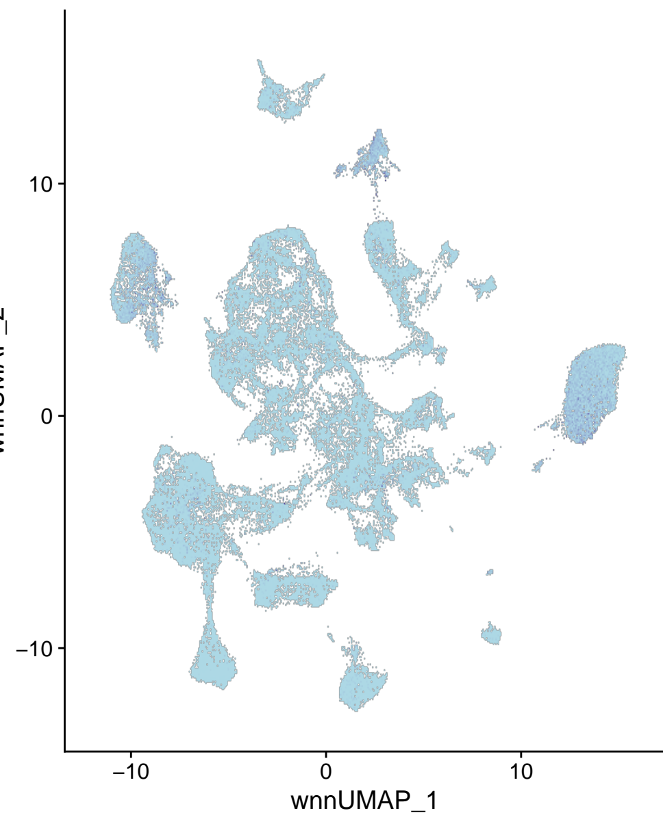
chr14-25740144-25740643
