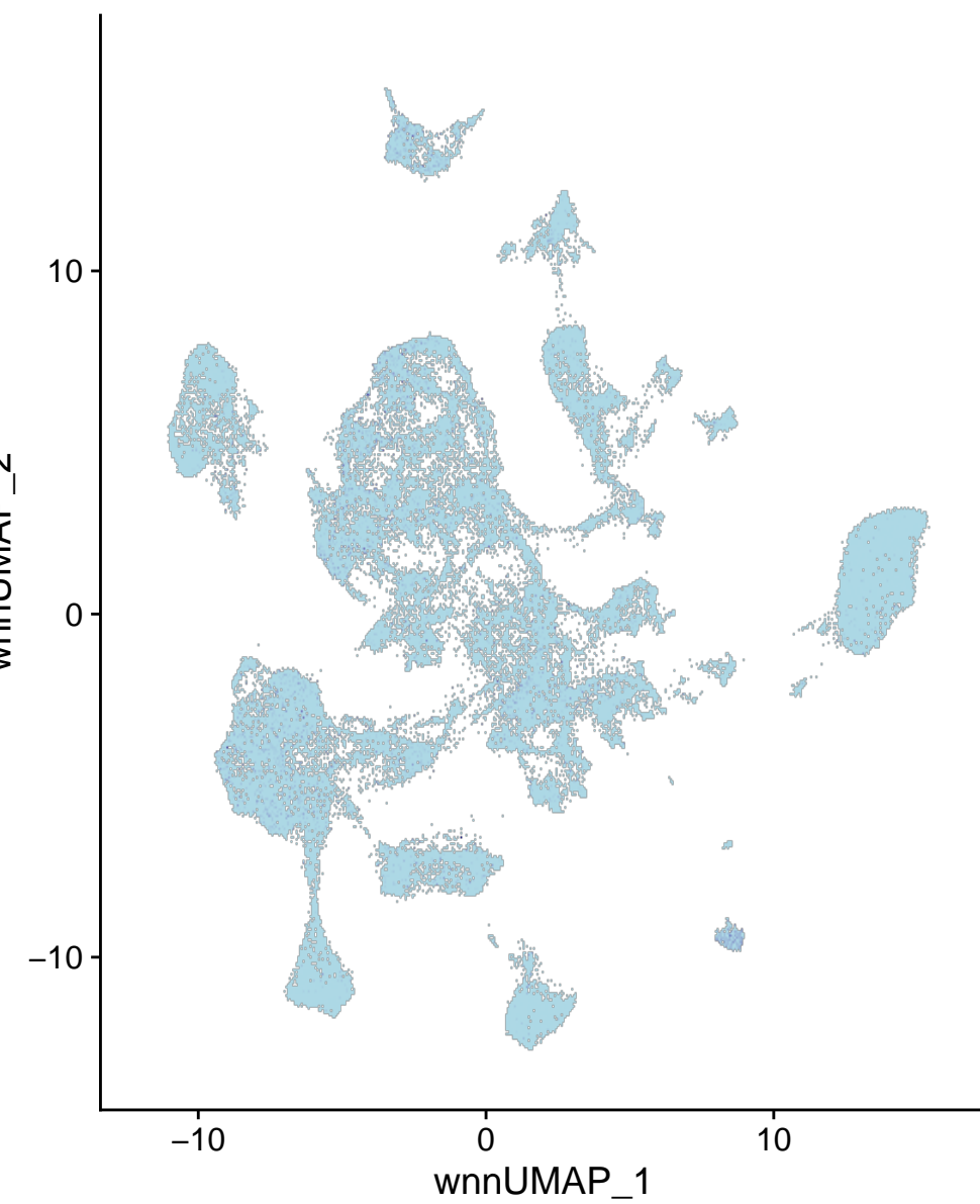
chr3-109917827-109918326
