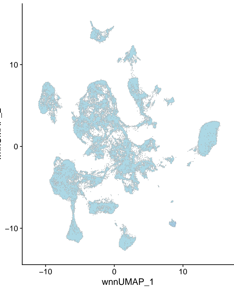
chr12-70157582-70158081
