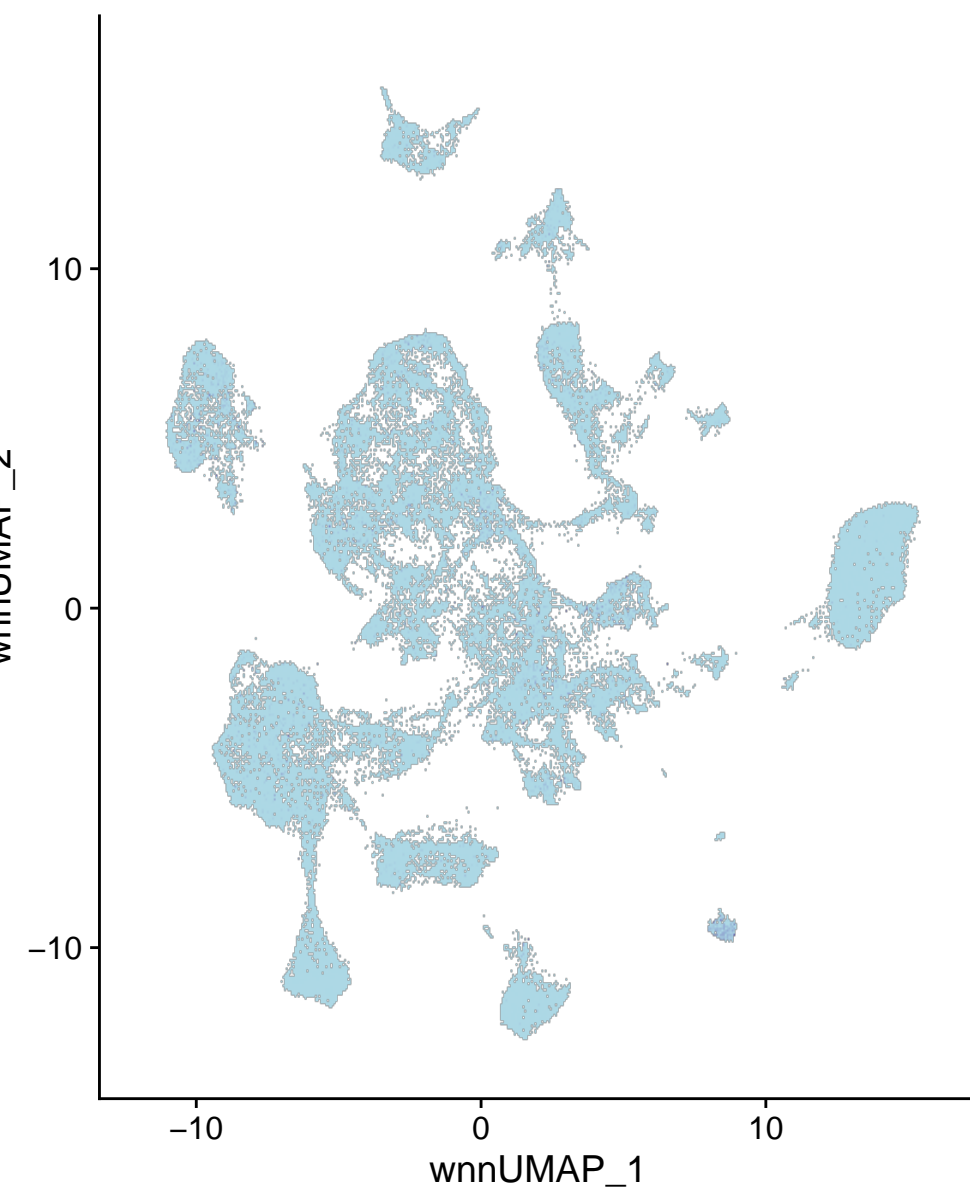
chr12-100123037-100123536
