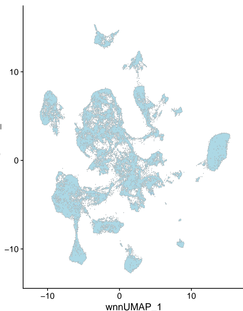
chr1-45425862-45426361
