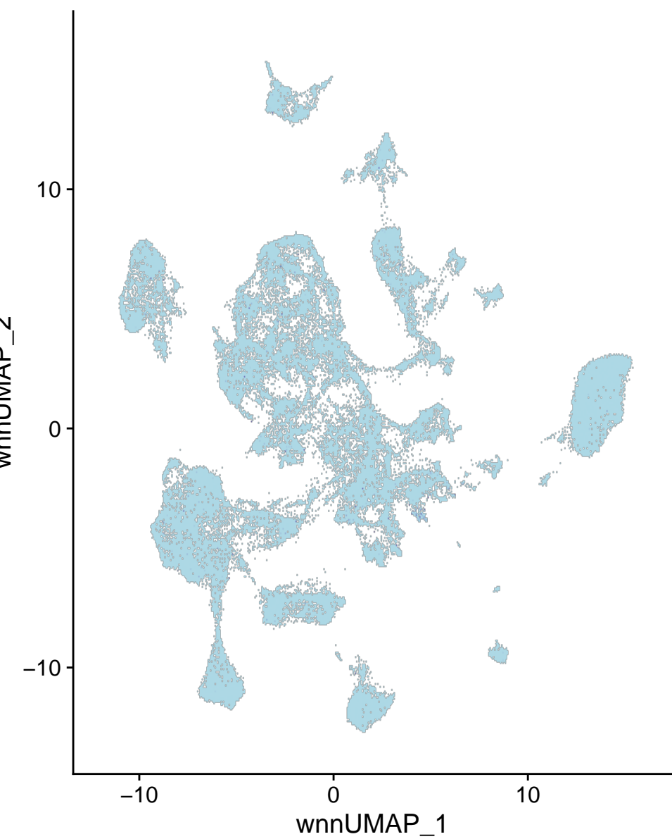
chr11-91056968-91057467
