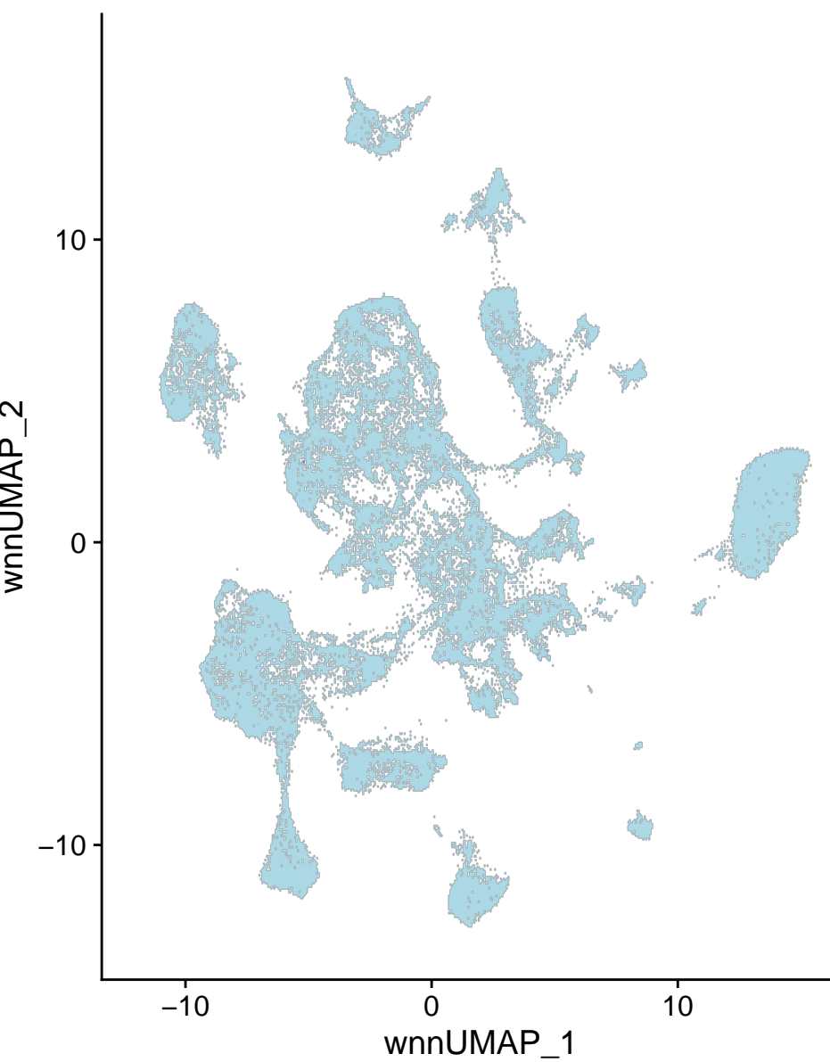
chr11-91034512-91035011
