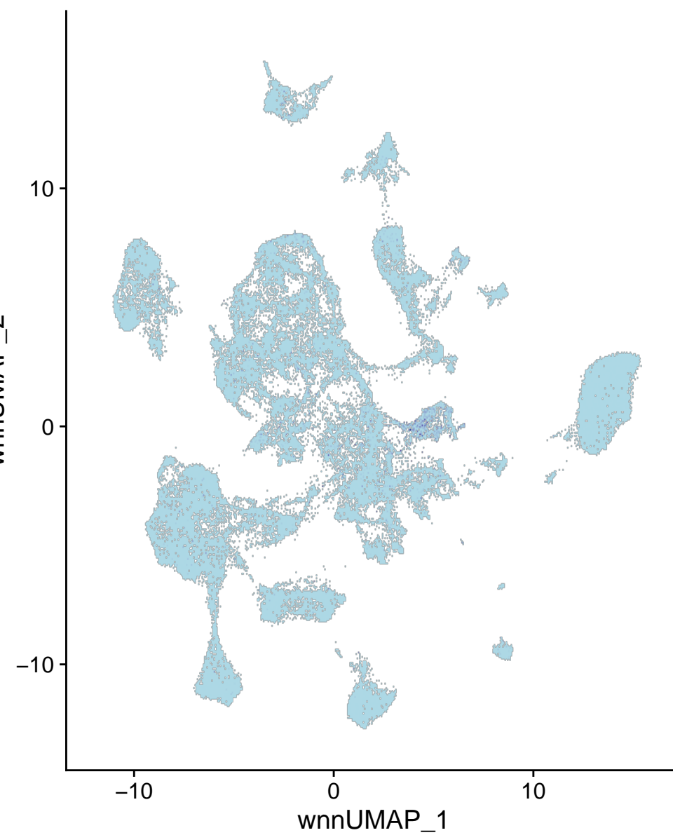
chr11-61098017-61098516
