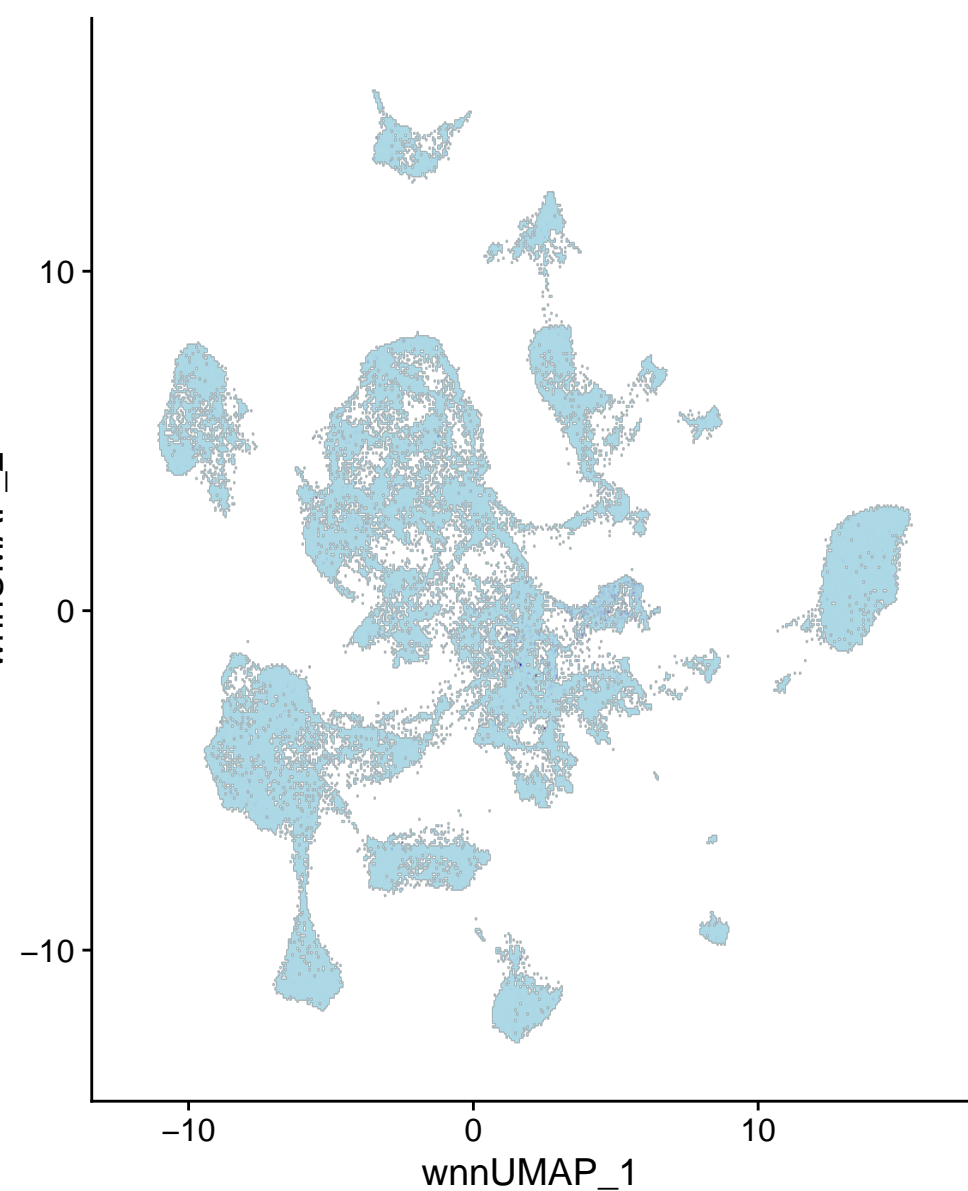
chr13-111061426-111061925
