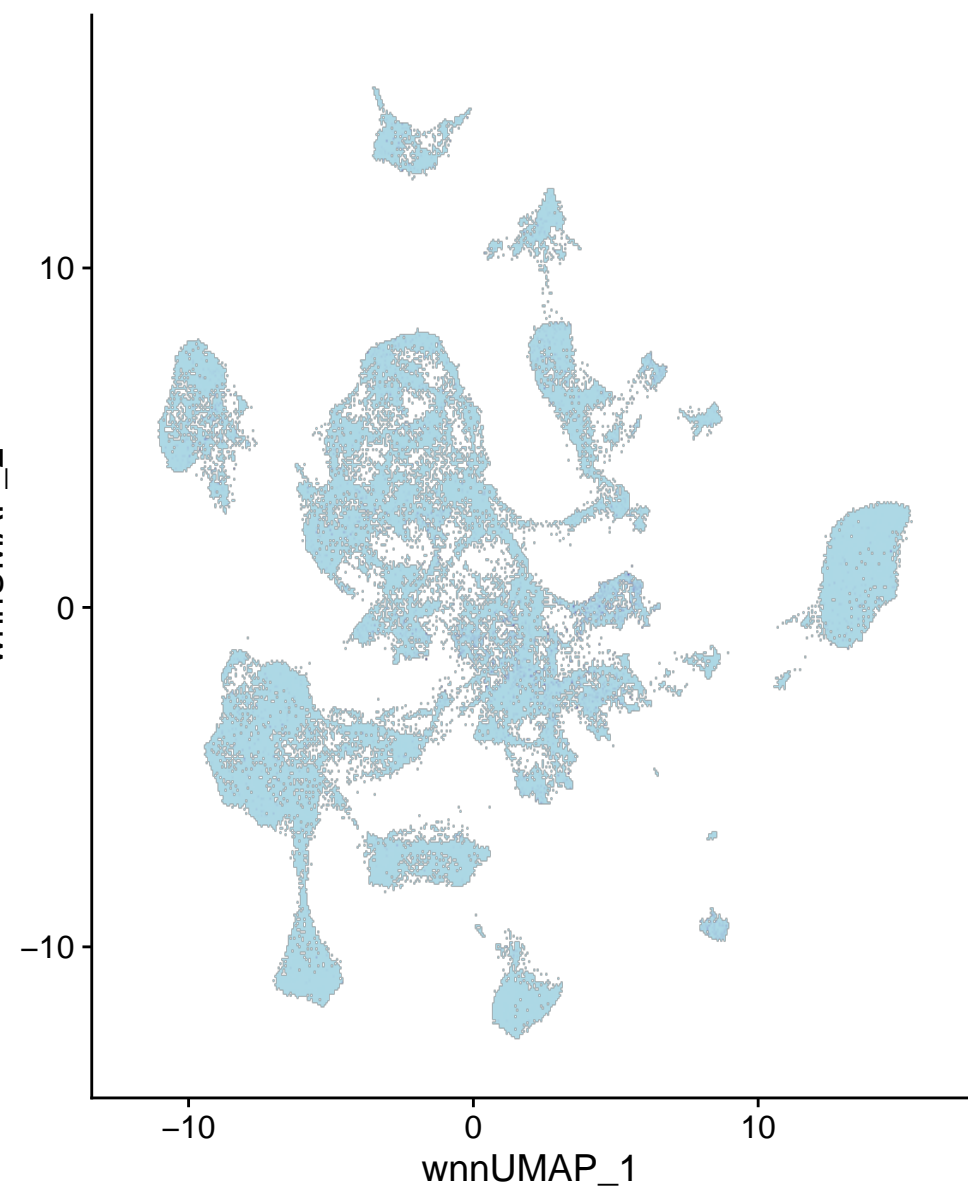
chr13-111061426-111061925
