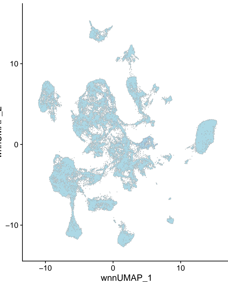
chr14-120877123-120877622
