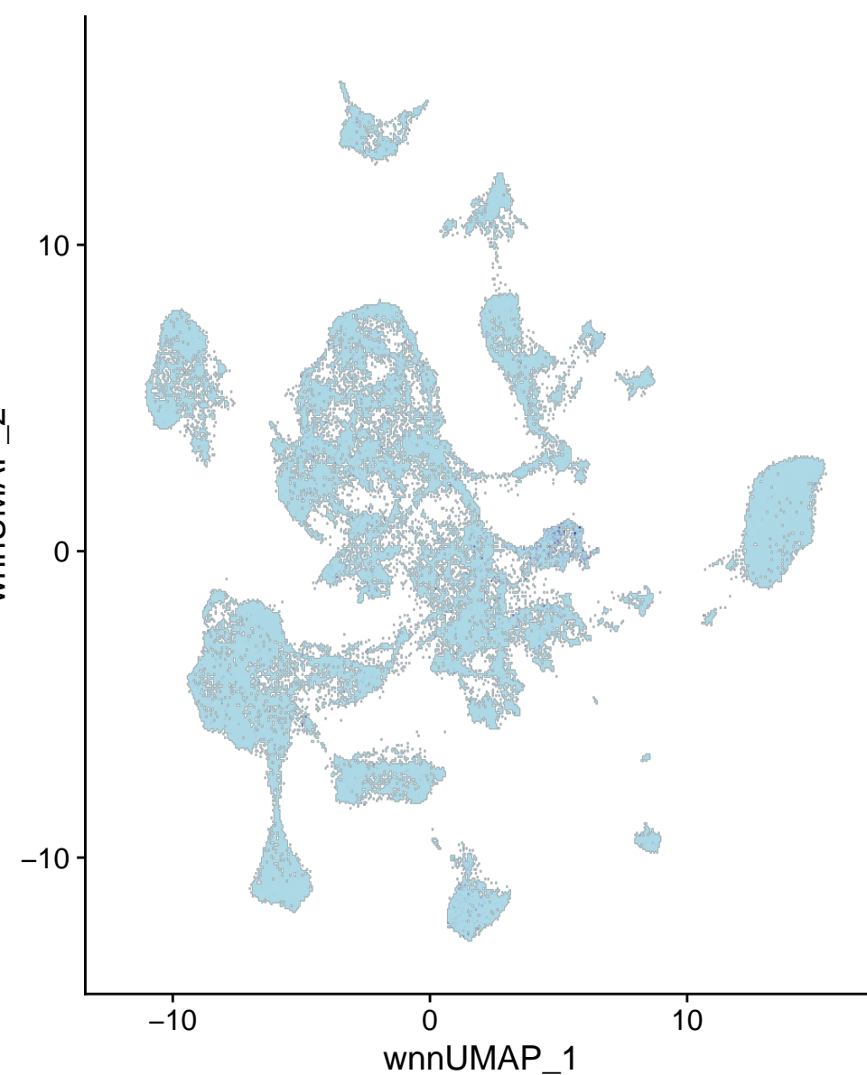
chr14-120877123-120877622
