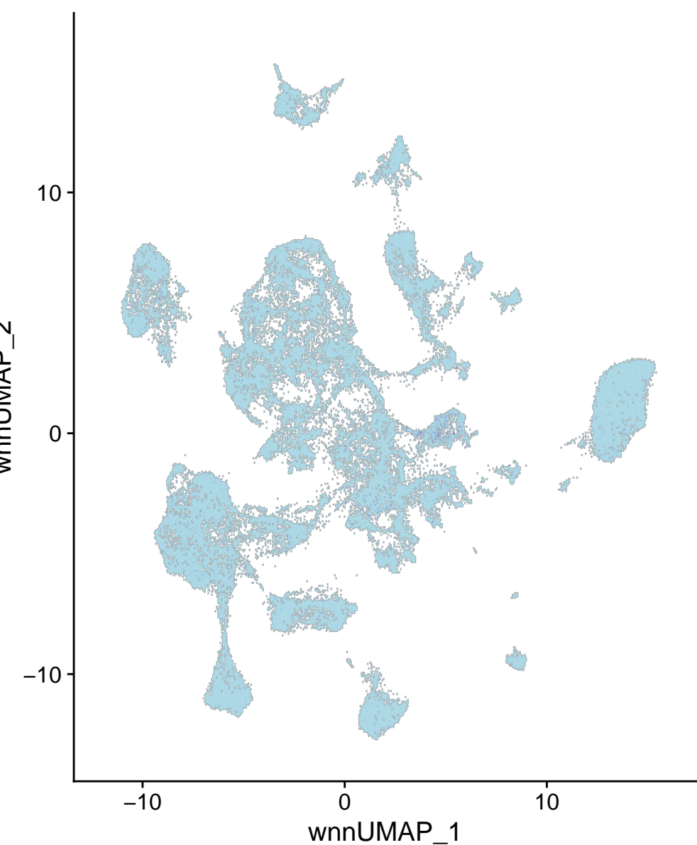
chr12-100831602-100832101
