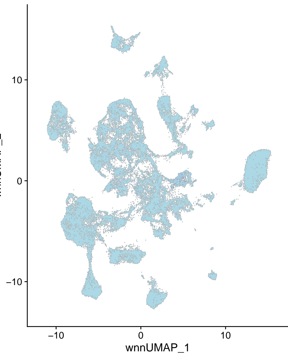
chr18-38869938-38870437
