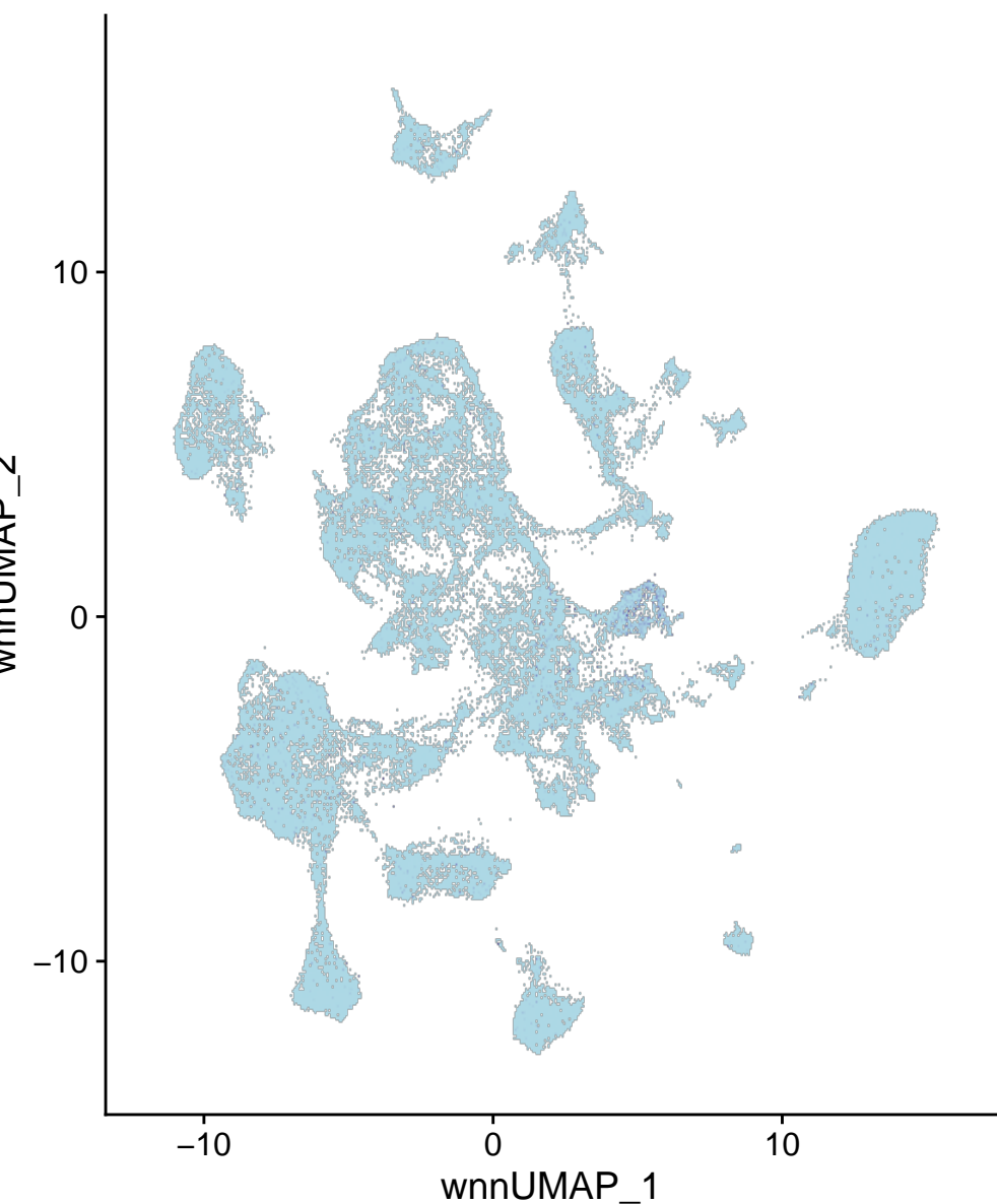
chr12-100831602-100832101
