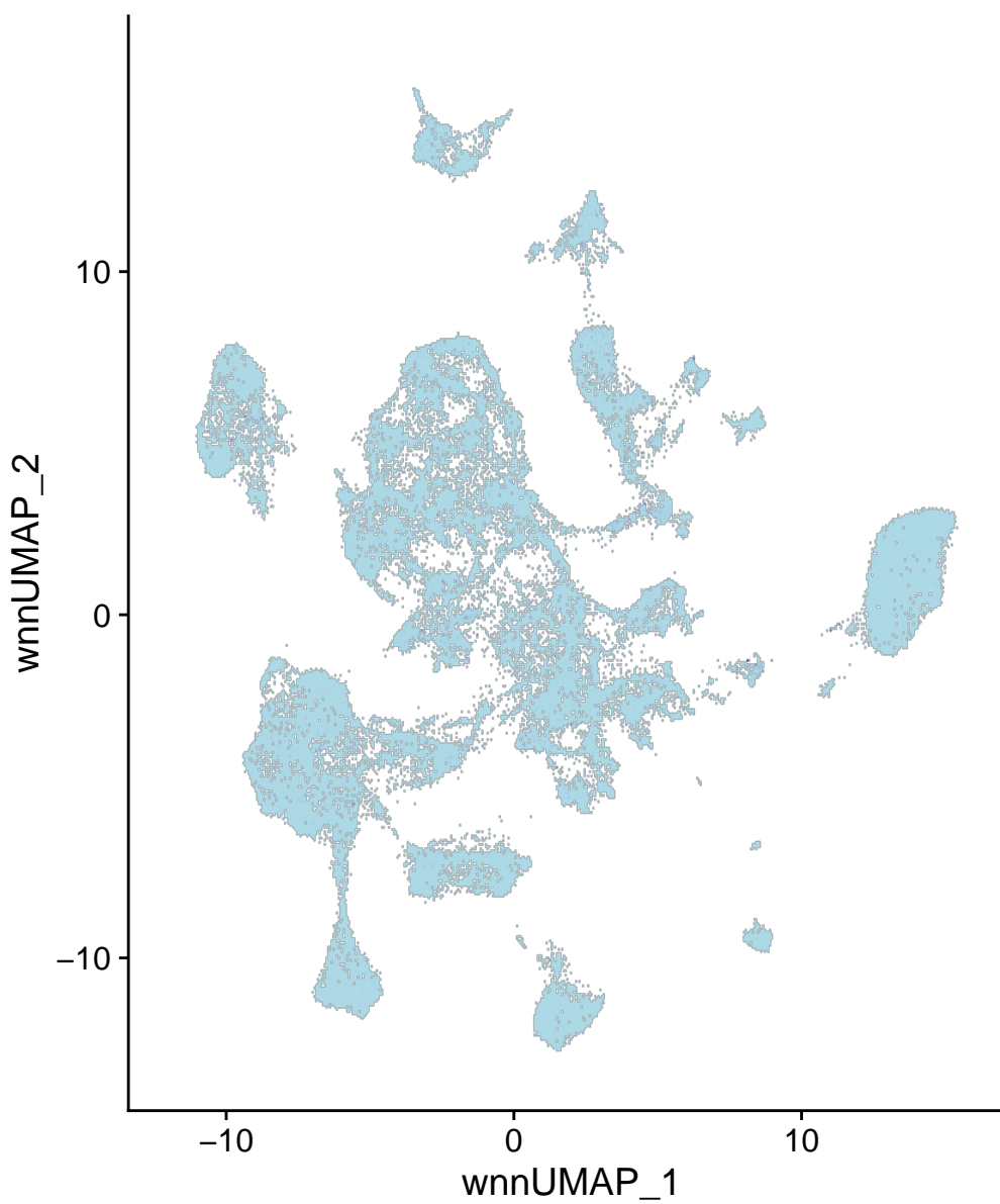
chr2-115249933-115250432
