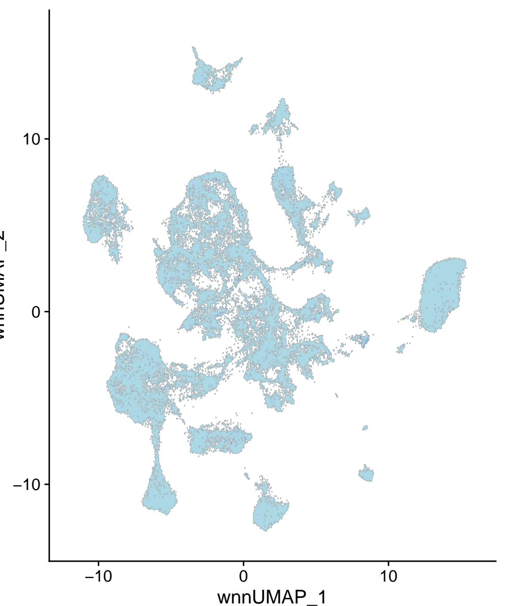
chr16-73244988-73245487
