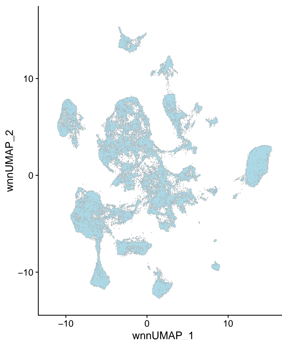
chr1-137838175-137838674
