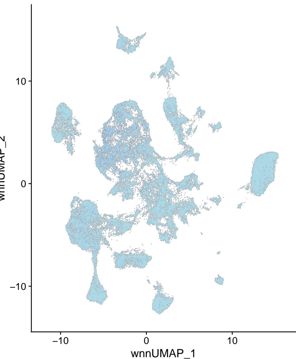
chr5-122615435-122615934
