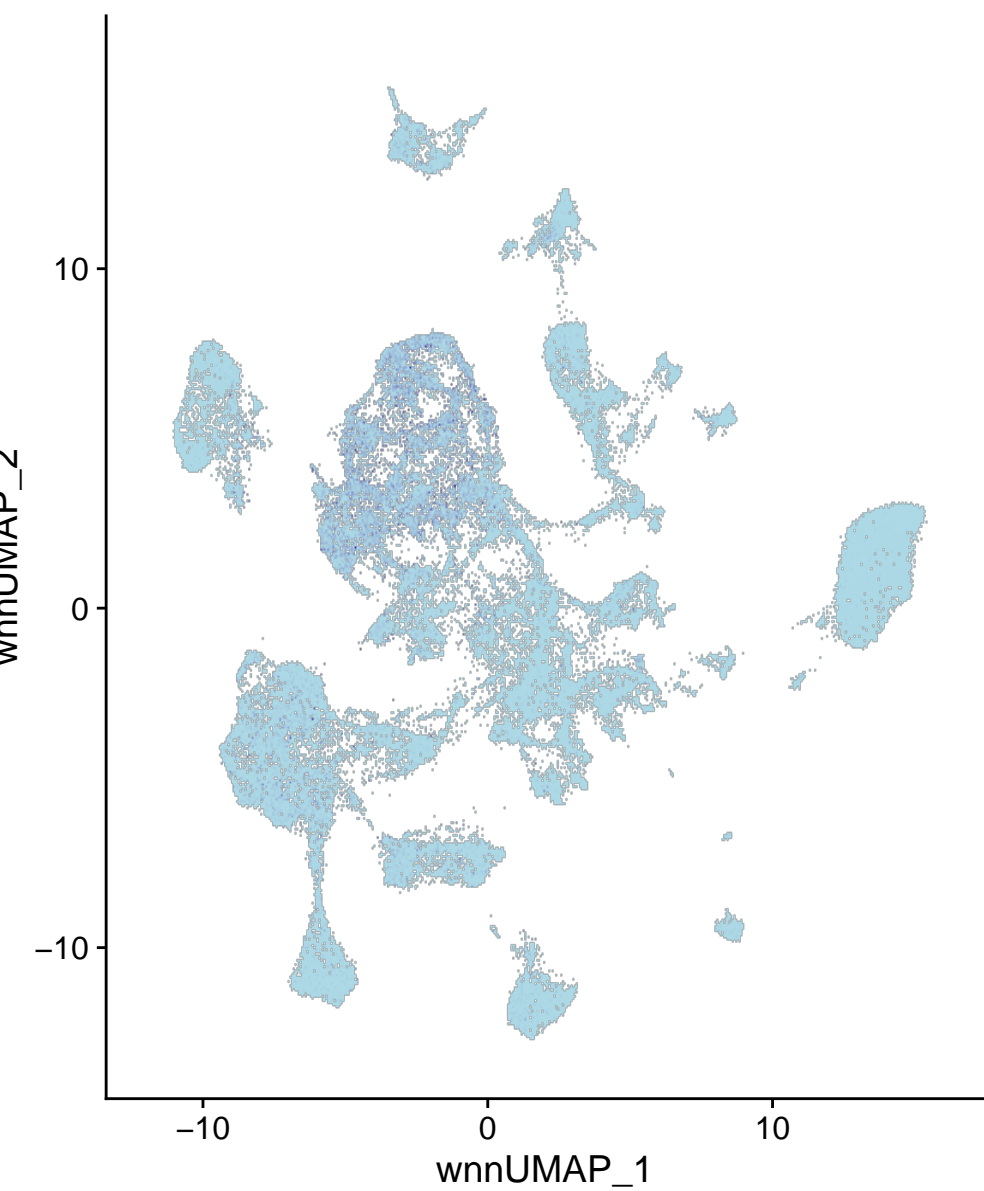
chr19-26795603-26796102
