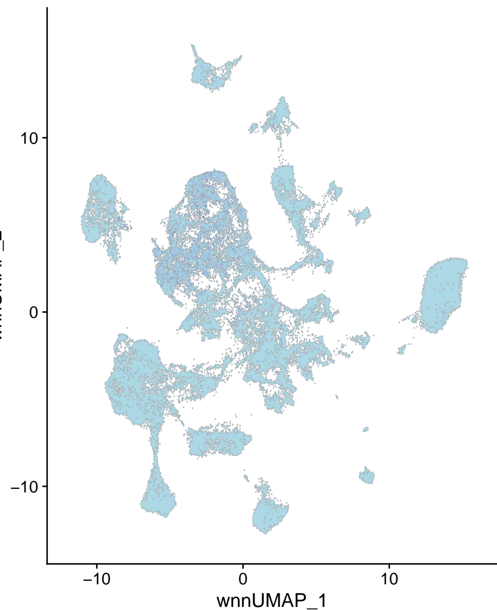
chr18-74515636-74516135
