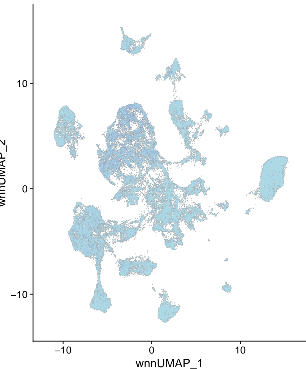
chr12-70291042-70291541
