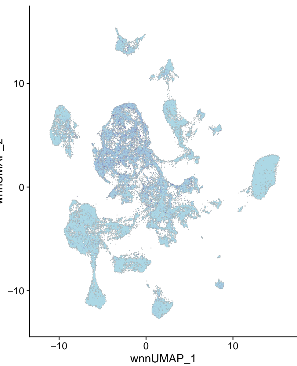
chr11-66694667-66695166
