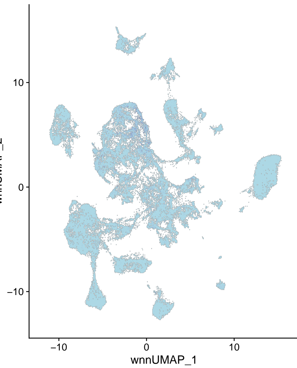
chr2-166100804-166101303
