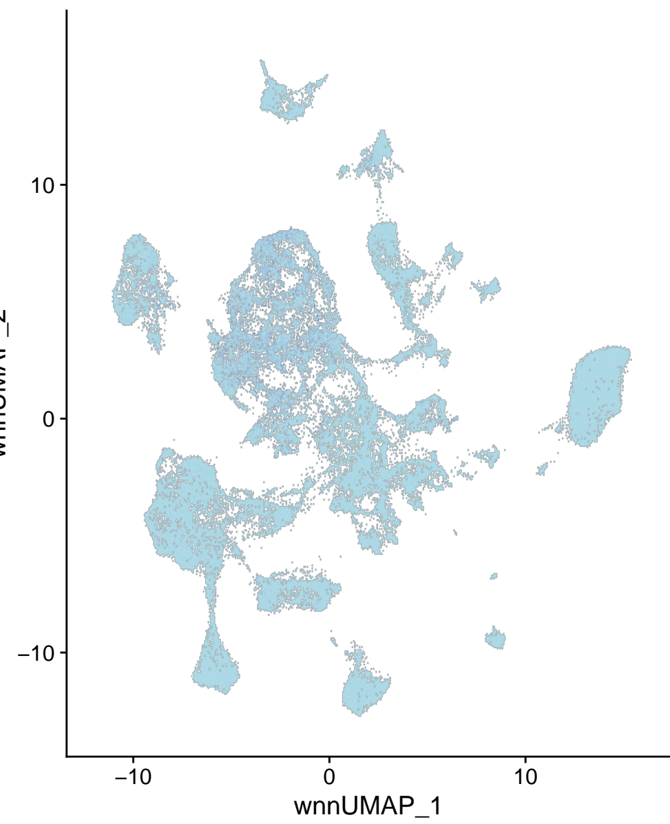
chr2-164432587-164433086
