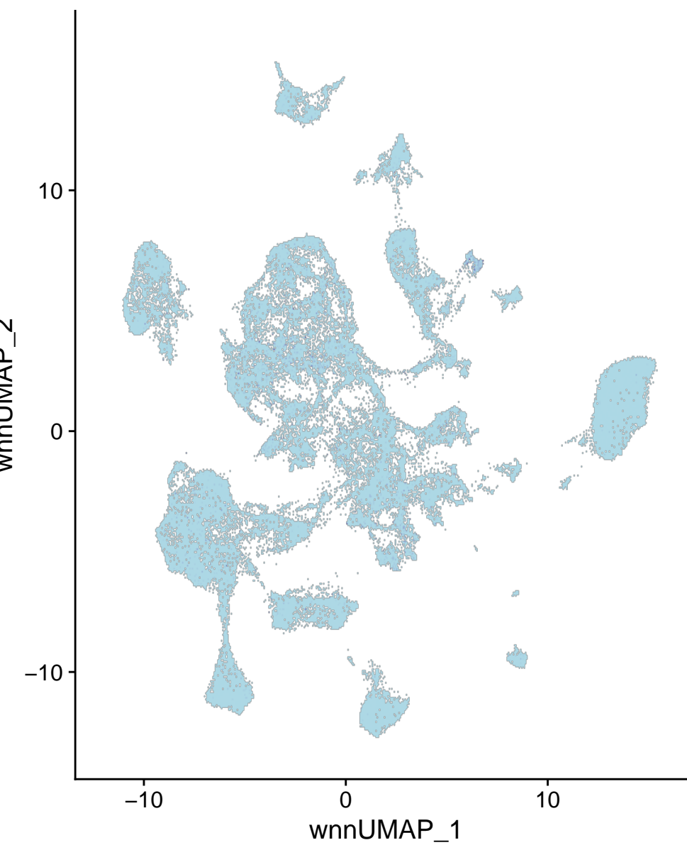
chr13-24054976-24055475
