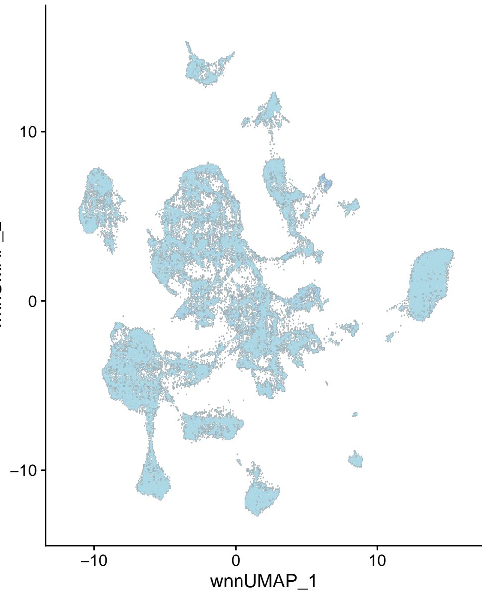
chr17-54223410-54223909
