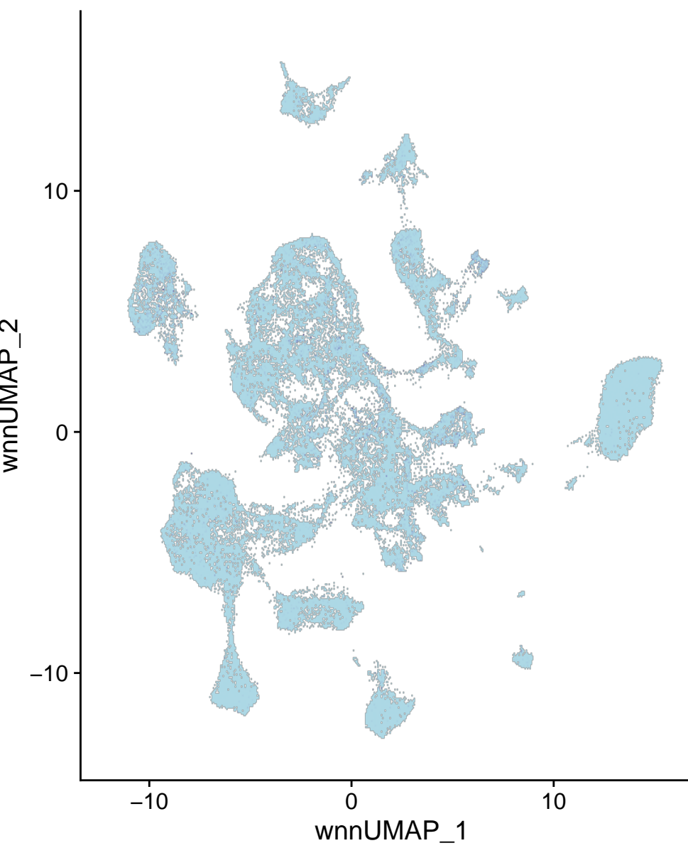
chr4-139995778-139996277
