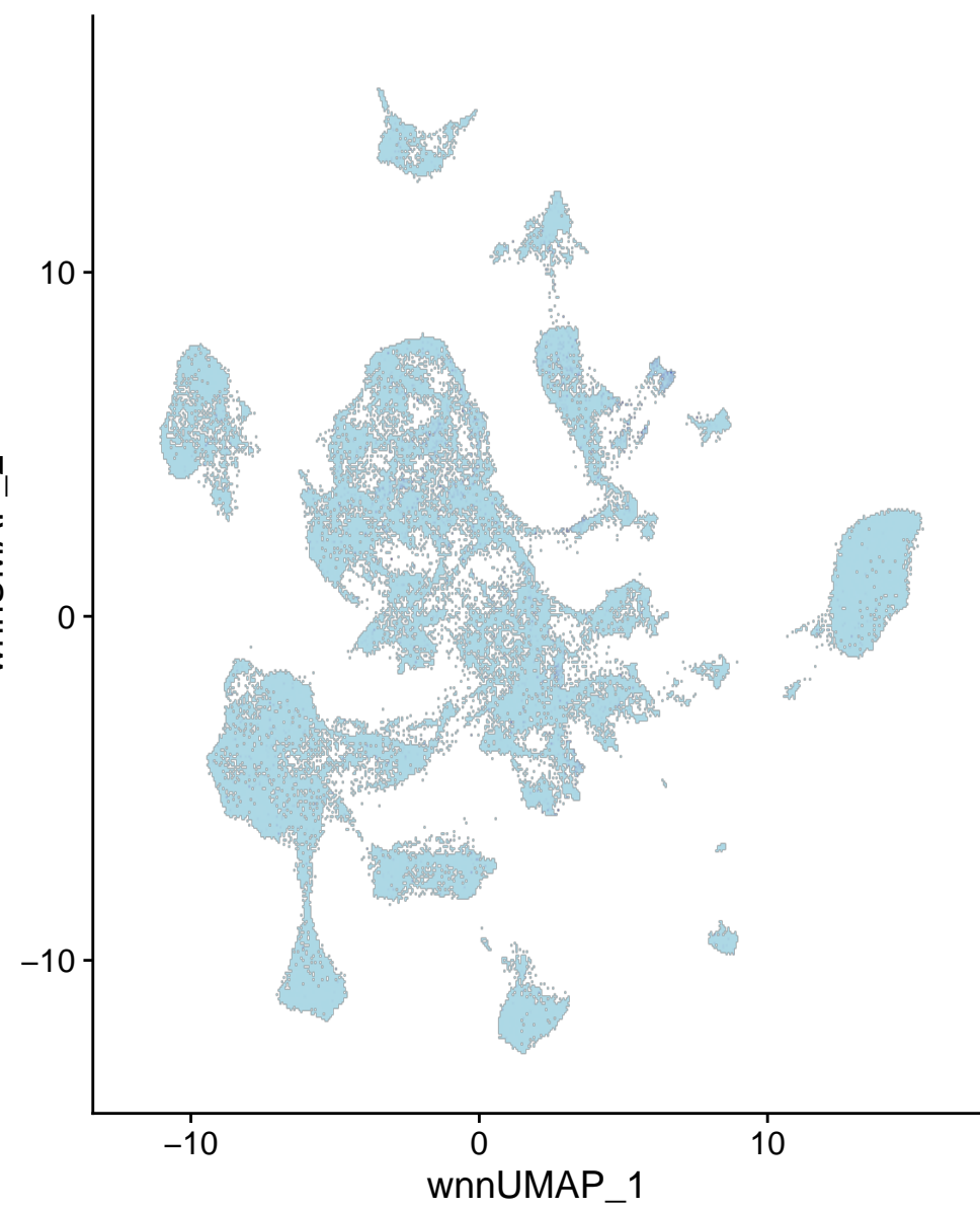
chr6-91745972-91746471
