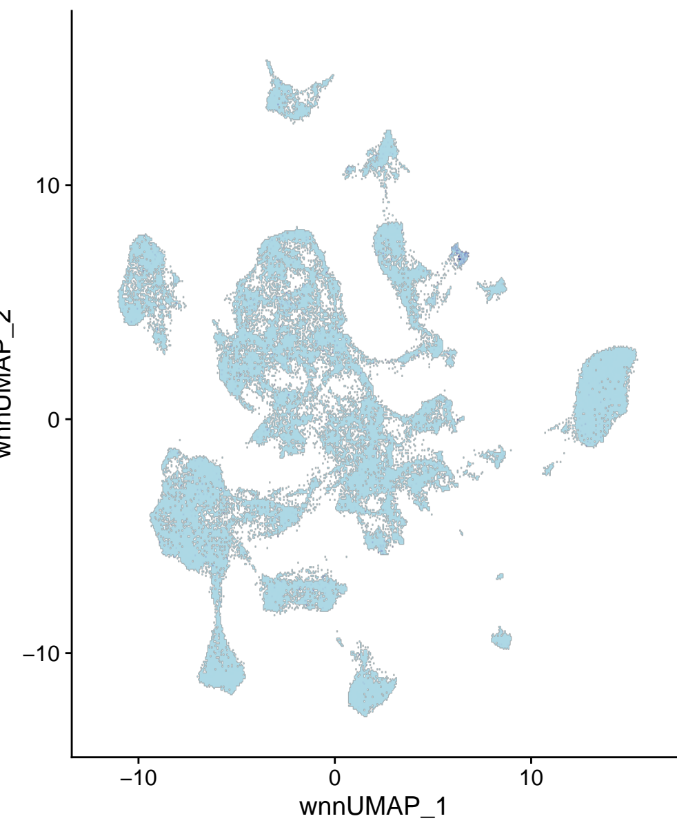
chr14-24828952-24829451
